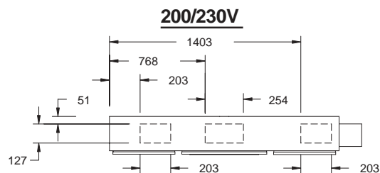
VIEW SHOWING CUSTOMER POWER ENTRY LOCATIONS ON UNDERSIDE OF PANEL
