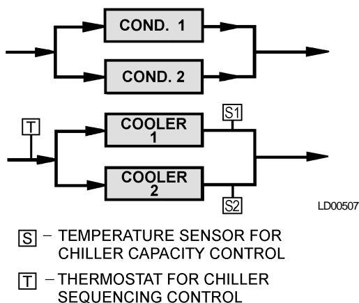
FIG. 1 – PARALLEL COOLERS PARALLEL CONDENSERS
