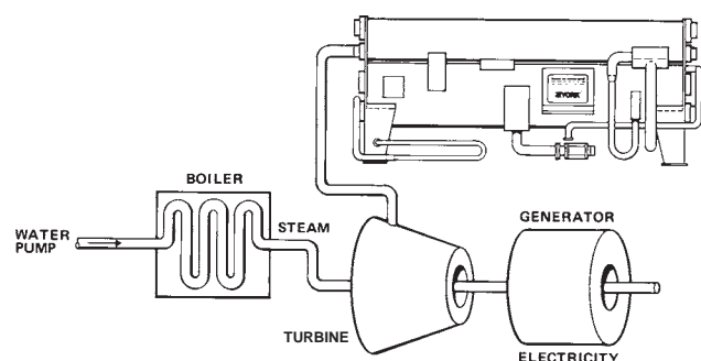
COGENERATION
