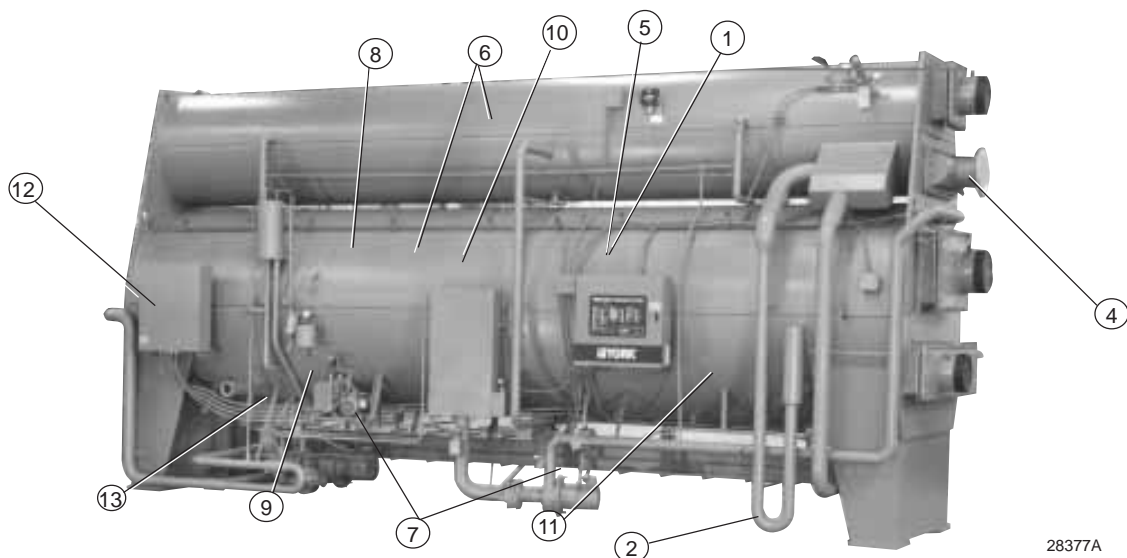
FIG. 1 – MILLENNIUM SINGLE-STAGE ABSORPTION CHILLER RELIABILITY FEATURES
