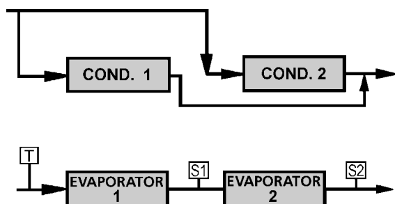
FIG. 2 – SERIES EVAPORATORS PARALLEL CONDENSERS
