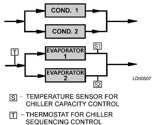
FIG. 1 – PARALLEL EVAPORATORS PARALLEL CONDENSERS
