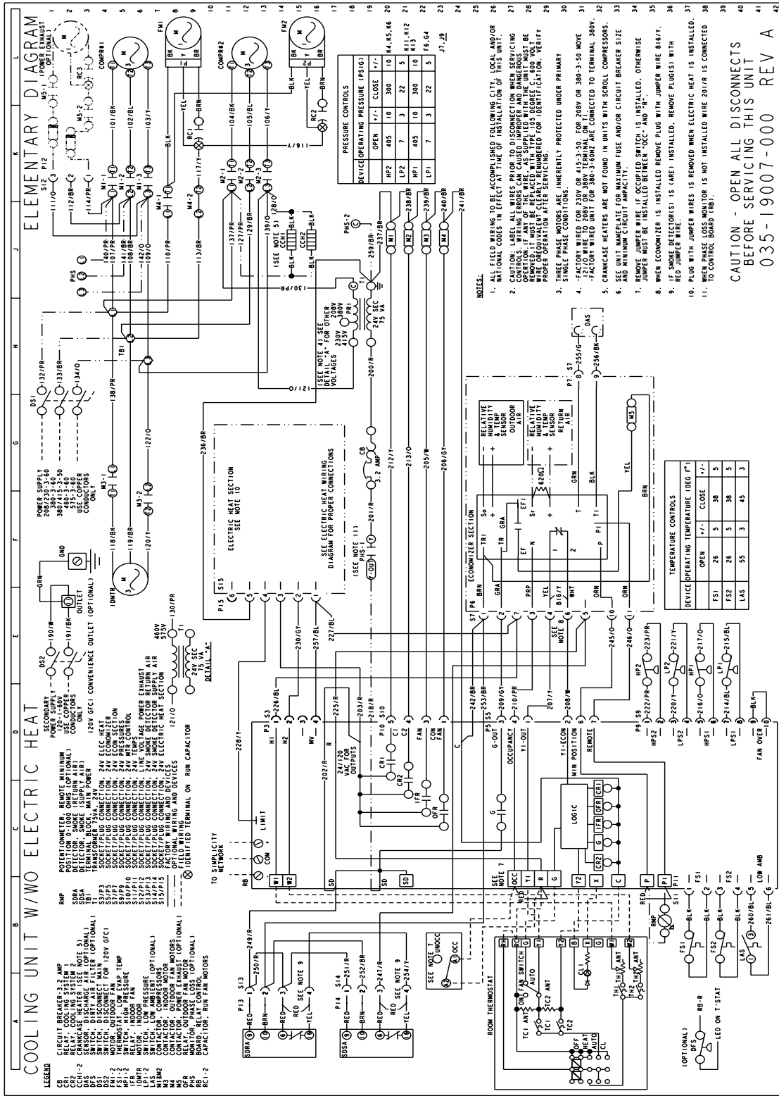
FIGURE 14 - COOLING UNIT WITH/WITHOUT ELECTRIC HEAT WIRING DIAGRAM
