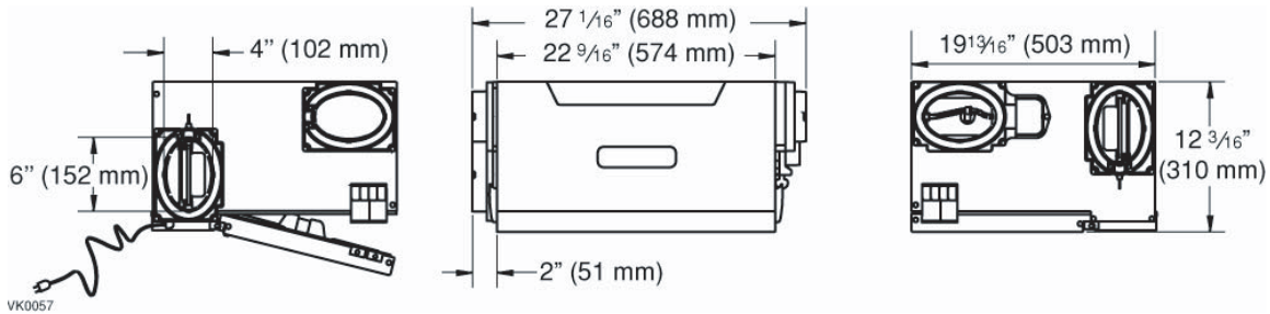
Fig. 2 - HRVCCSHA Unit Dimensions
