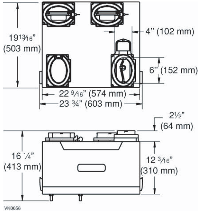
Fig. 3 - HRVCCSVA Unit Dimensions
